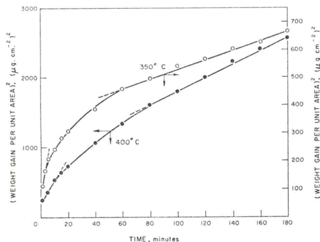
Fig. 9. Parabolic plot of data from the high pressure oxidation at 350° and 400°C.
